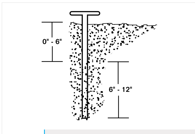
Figure 5. A sampling tube or auger is needed to collect subsurface samples.
